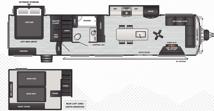
39/391FLSL WEIGHT 12220 LENGTH 42' 11"
