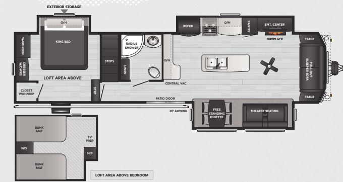
39/391LOFT WEIGHT 12568 LENGTH 40' 8"
