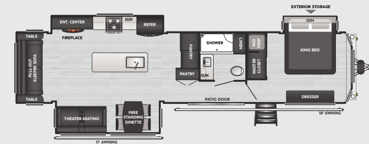
39/391RS WEIGHT TBD LENGTH 40' 11"
