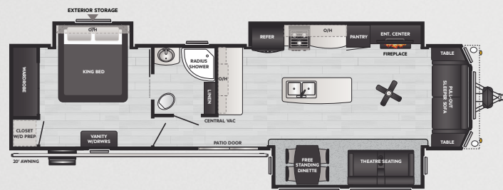
39/391MKTS WEIGHT 11820 LENGTH 40' 8"
